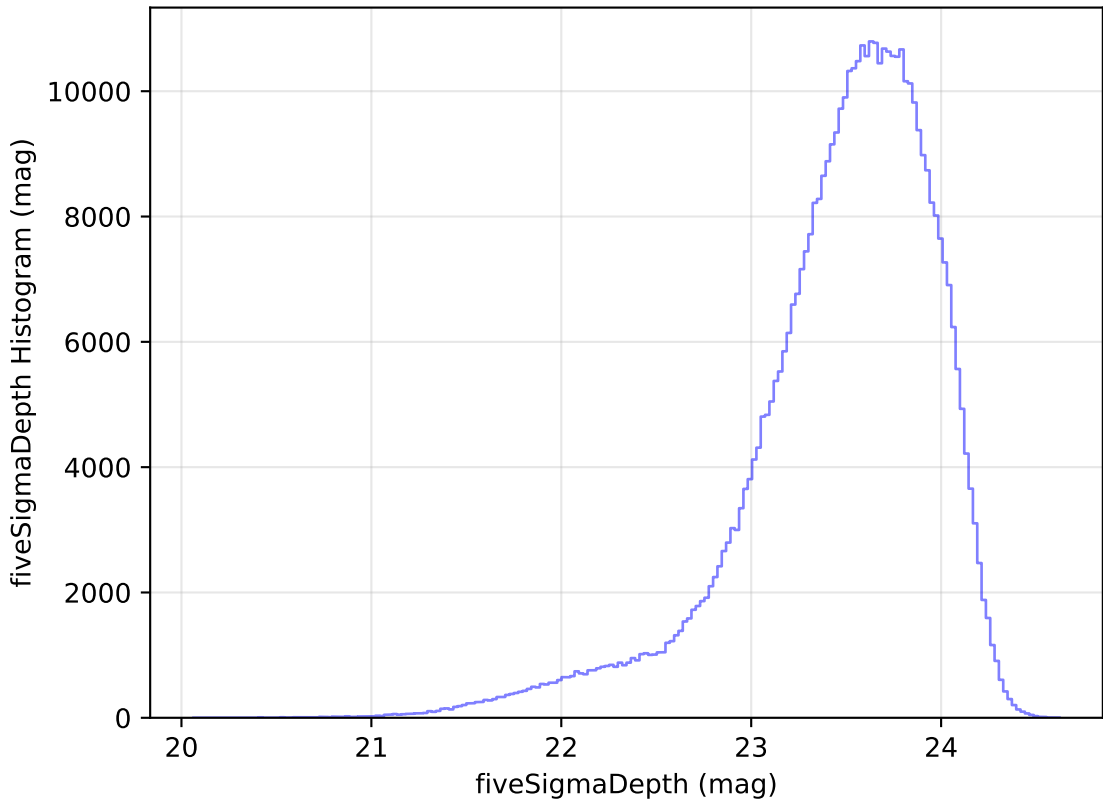
too_elab_r32_d3_griz_v3.4_10yrs All sky i band: fiveSigmaDepth Histogram
