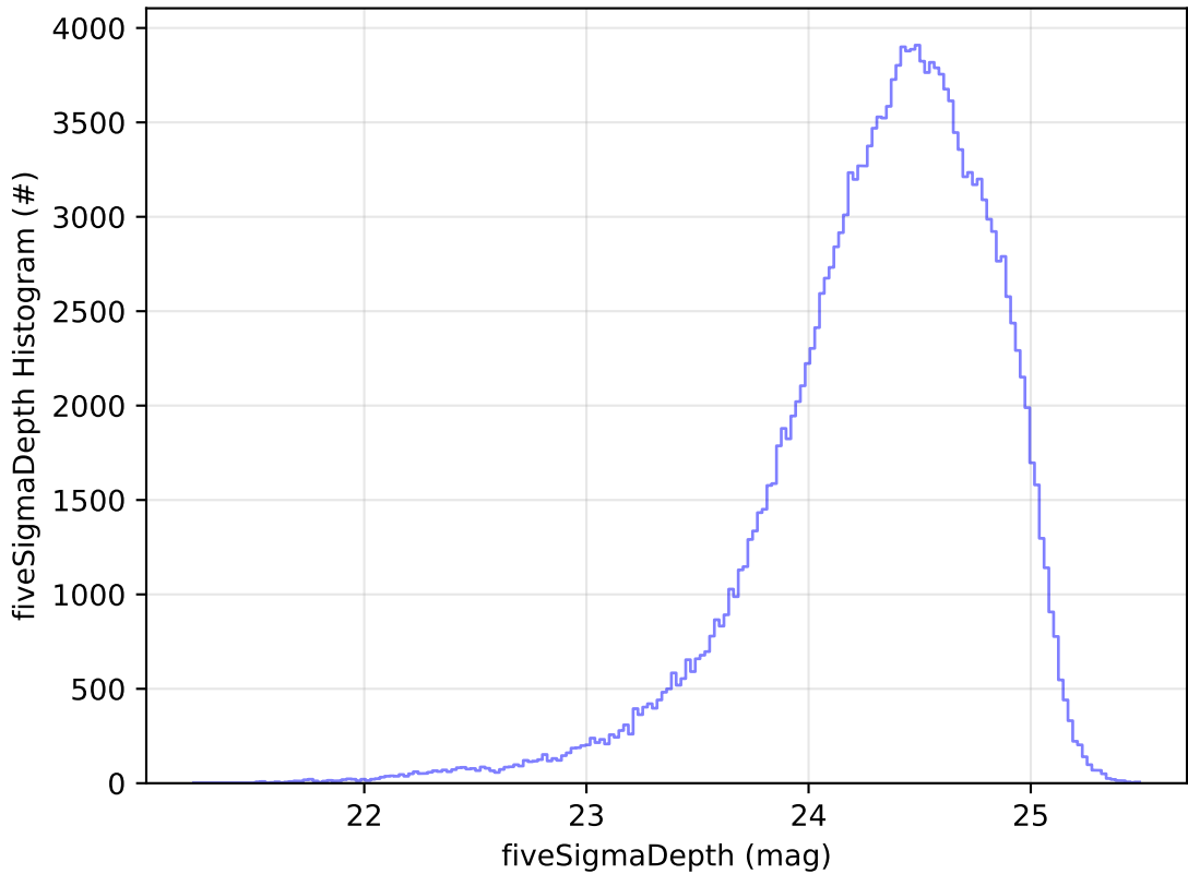
too_elab_r32_d3_griz_v3.4_10yrs All sky g band: fiveSigmaDepth Histogram
