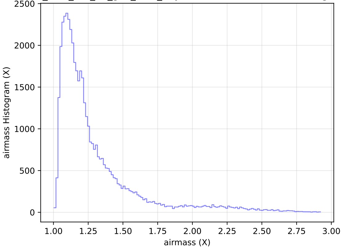
too_elab_r32_d3_griz_v3.4_10yrs Yr 1 z band: airmass Histogram
