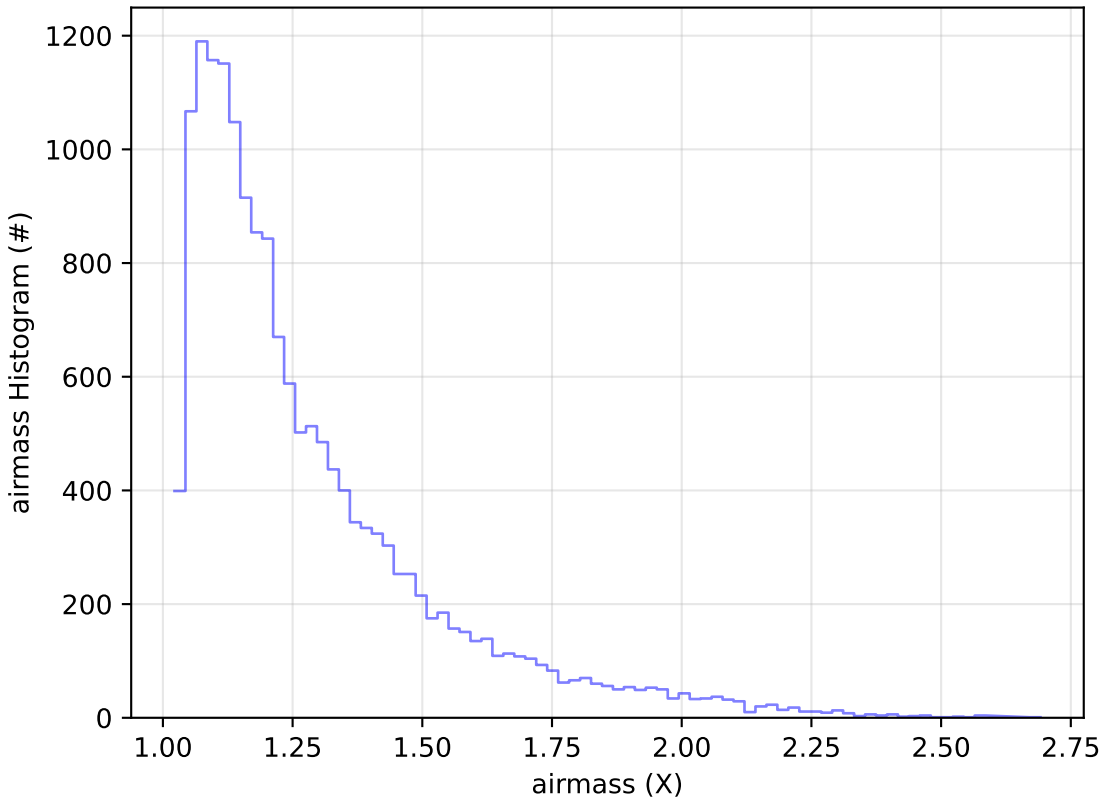
too_elab_r32_d3_griz_v3.4_10yrs Yr 1 u band: airmass Histogram
