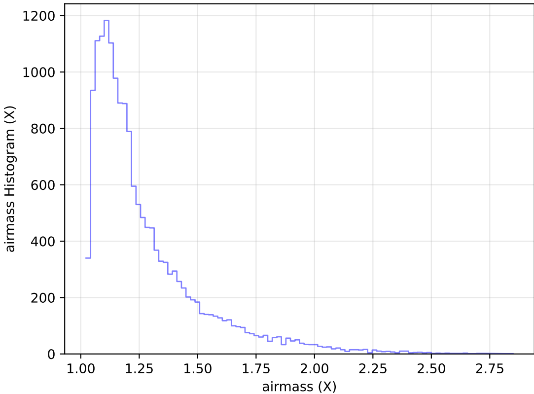
too_elab_r32_d3_griz_v3.4_10yrs Yr 1 u band: airmass Histogram
