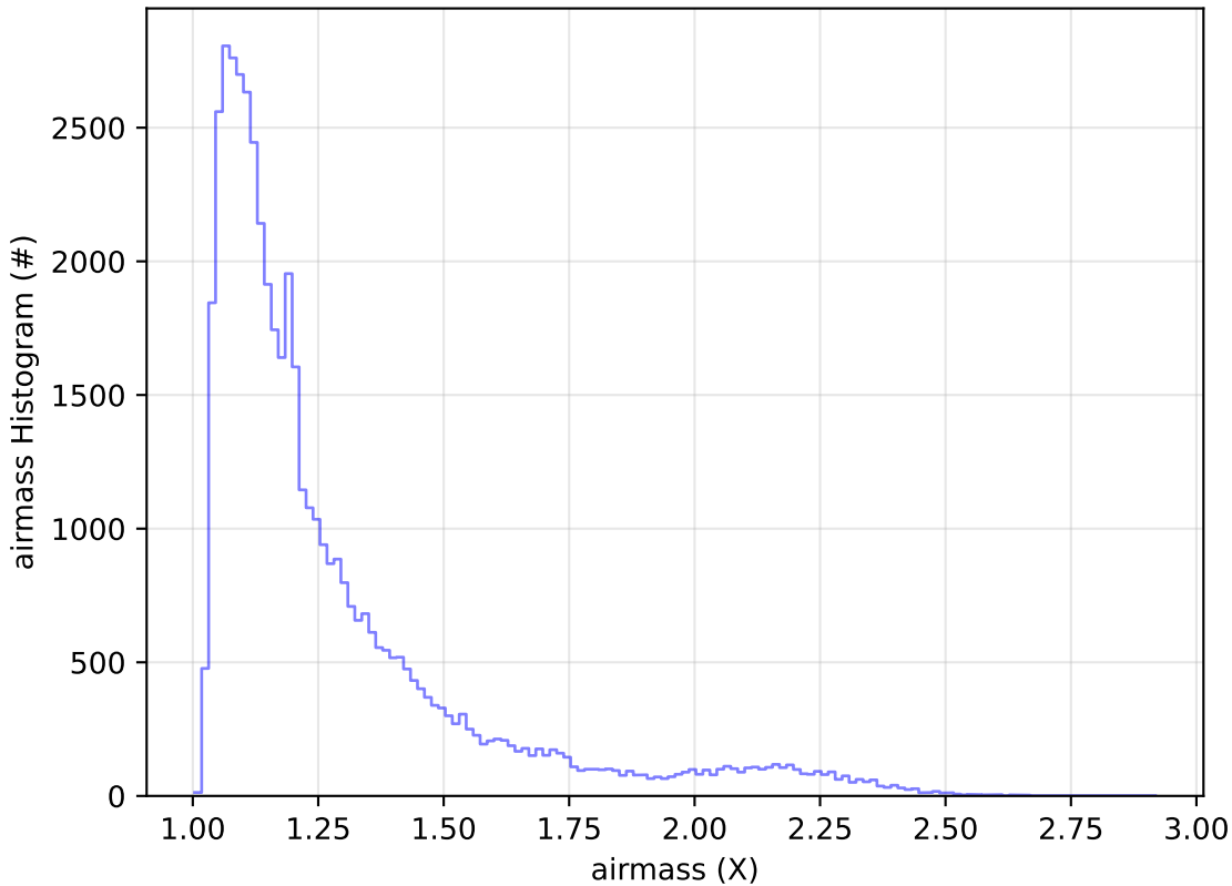
too_elab_r32_d3_griz_v3.4_10yrs Yr 1 r band: airmass Histogram
