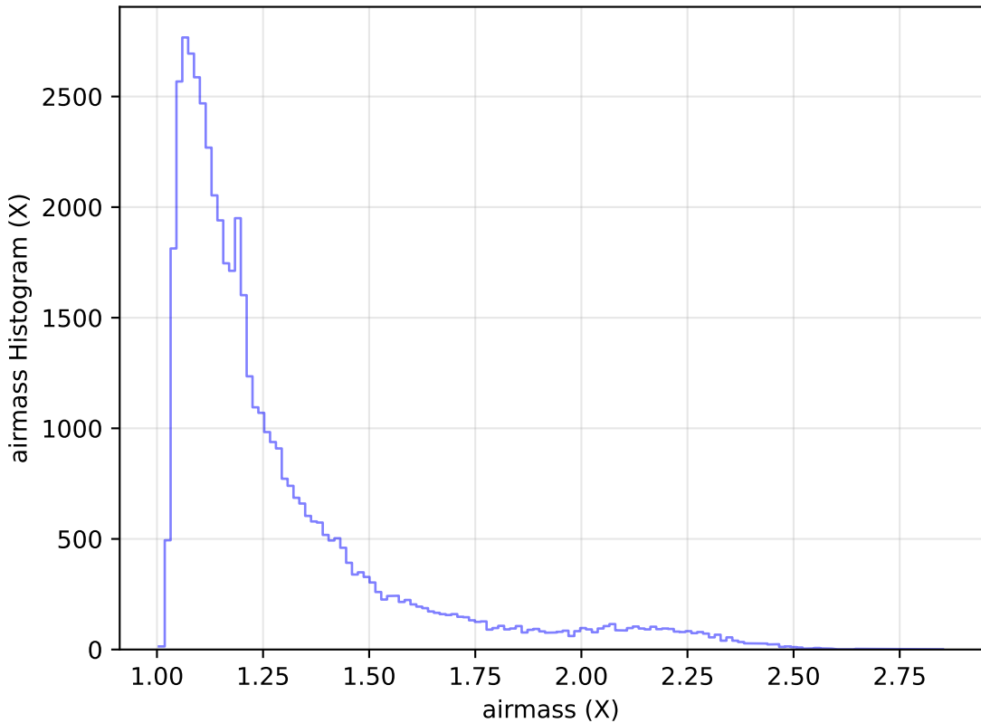
too_elab_r32_d3_griz_v3.4_10yrs Yr 1 r band: airmass Histogram
