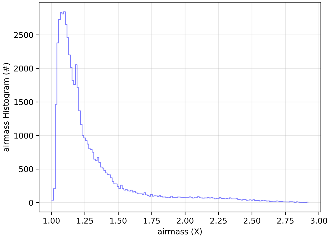
too_elab_r32_d3_griz_v3.4_10yrs Yr 1 i band: airmass Histogram
