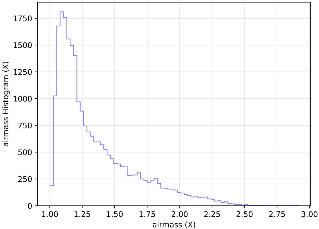
too_elab_r32_d3_griz_v3.4_10yrs Yr 1 g band: airmass Histogram
