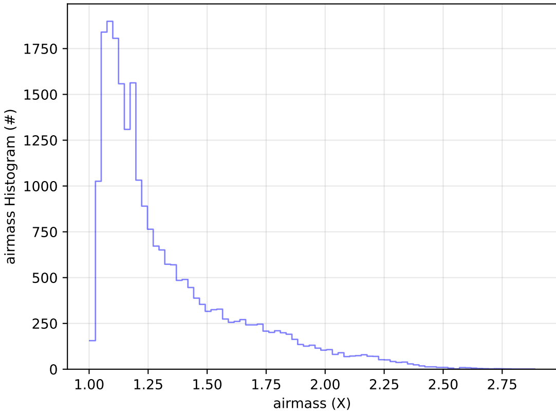
too_elab_r32_d3_griz_v3.4_10yrs Yr 1 g band: airmass Histogram
