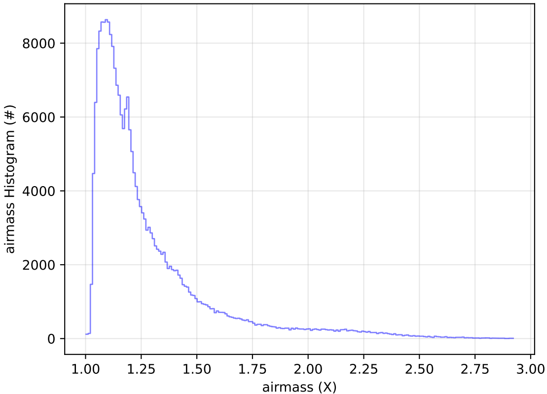
too_elab_r32_d3_griz_v3.4_10yrs Yr 1 all bands: airmass Histogram
