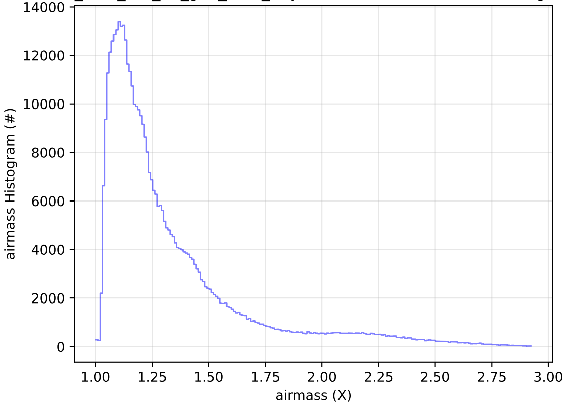
too_elab_r32_d3_griz_v3.4_10yrs WFD z band: airmass Histogram
