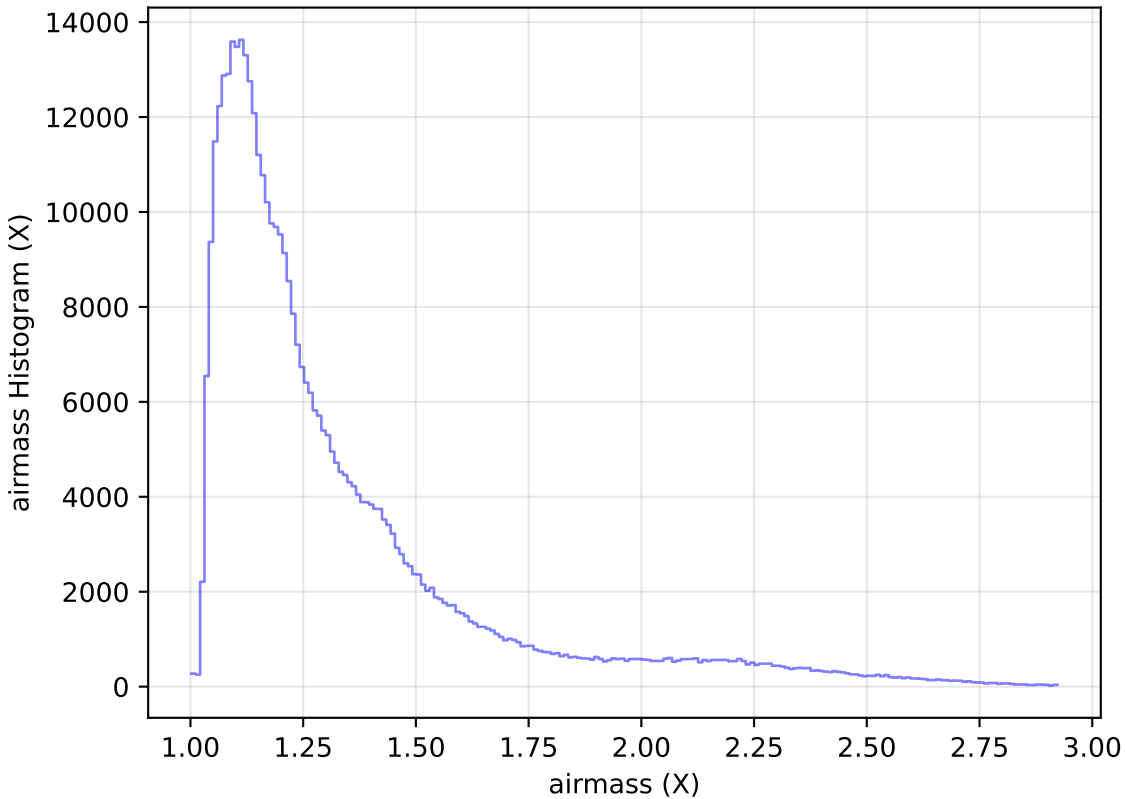
too_elab_r32_d3_griz_v3.4_10yrs WFD z band: airmass Histogram
