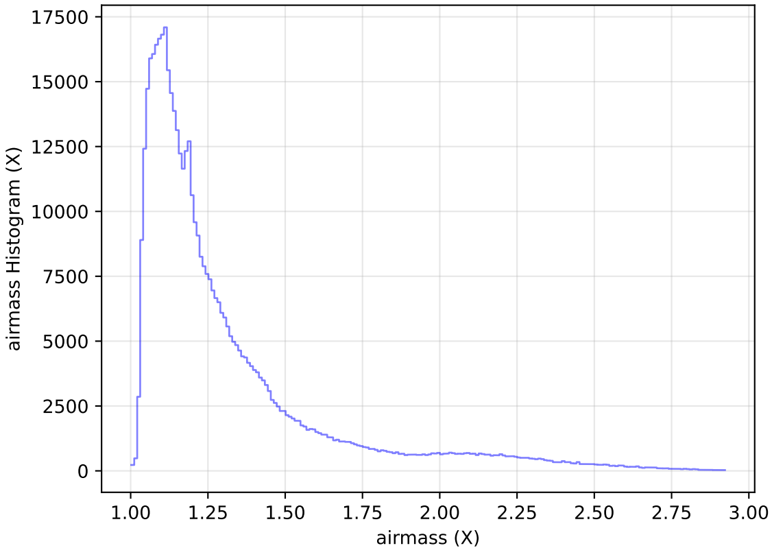
too_elab_r32_d3_griz_v3.4_10yrs WFD i band: airmass Histogram
