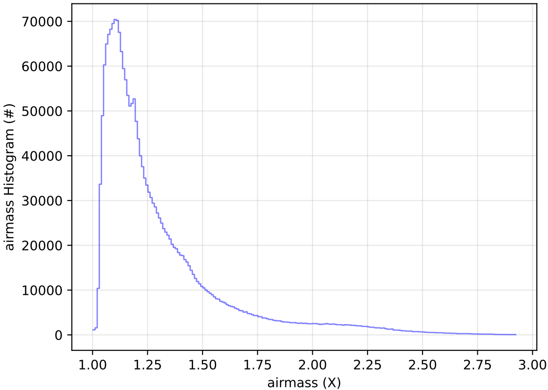
too_elab_r32_d3_griz_v3.4_10yrs WFD all bands: airmass Histogram
