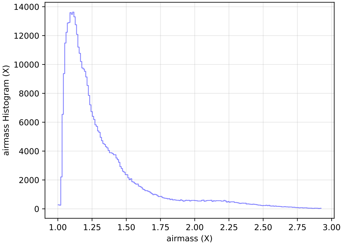
too_elab_r32_d3_griz_v3.4_10yrs All sky z band: airmass Histogram
