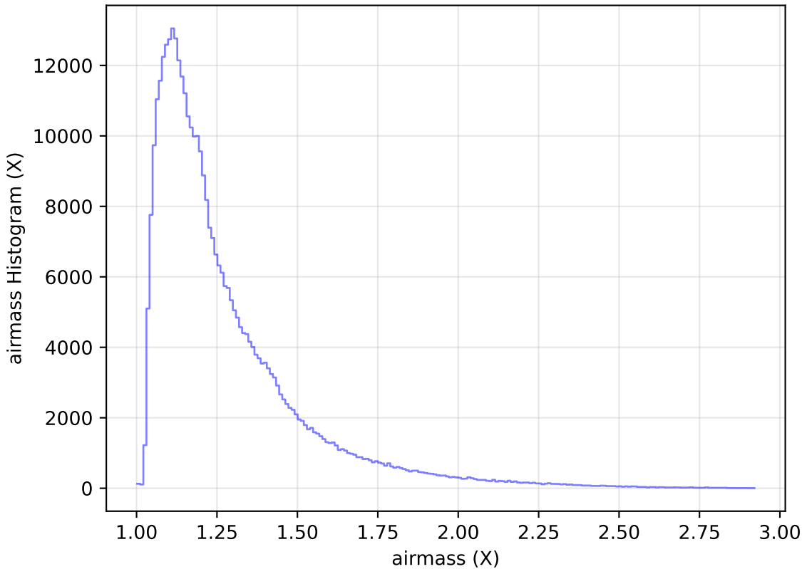
too_elab_r32_d3_griz_v3.4_10yrs All sky y band: airmass Histogram
