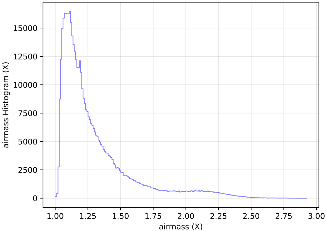
too_elab_r32_d3_griz_v3.4_10yrs All sky r band: airmass Histogram
