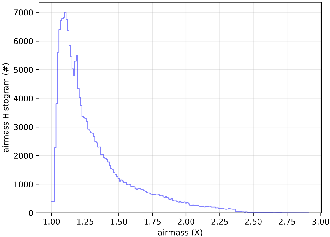
too_elab_r32_d3_griz_v3.4_10yrs All sky g band: airmass Histogram
