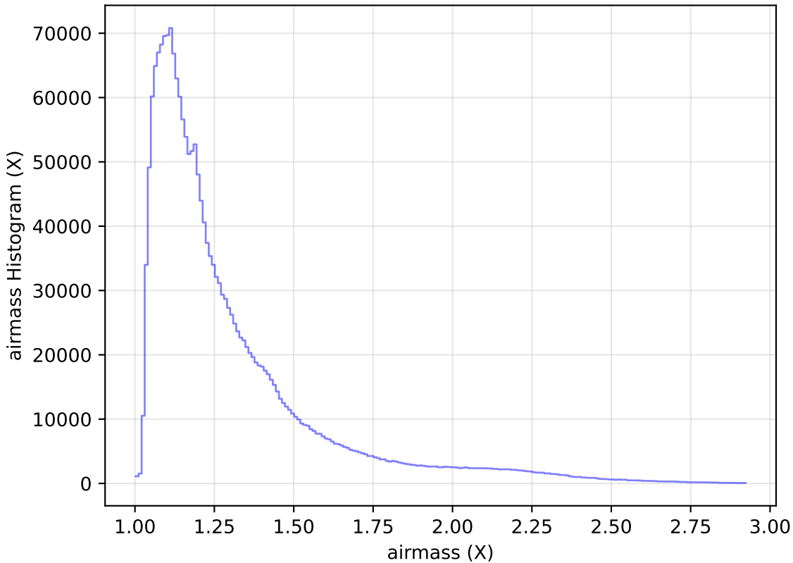
too_elab_r32_d3_griz_v3.4_10yrs All sky all bands: airmass Histogram
