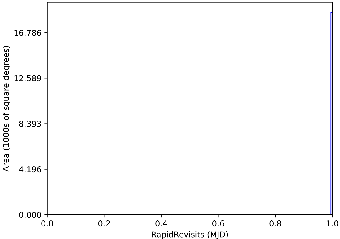
too_elab_r32_d3_griz_v3.4_10yrs WFD: RapidRevisits
