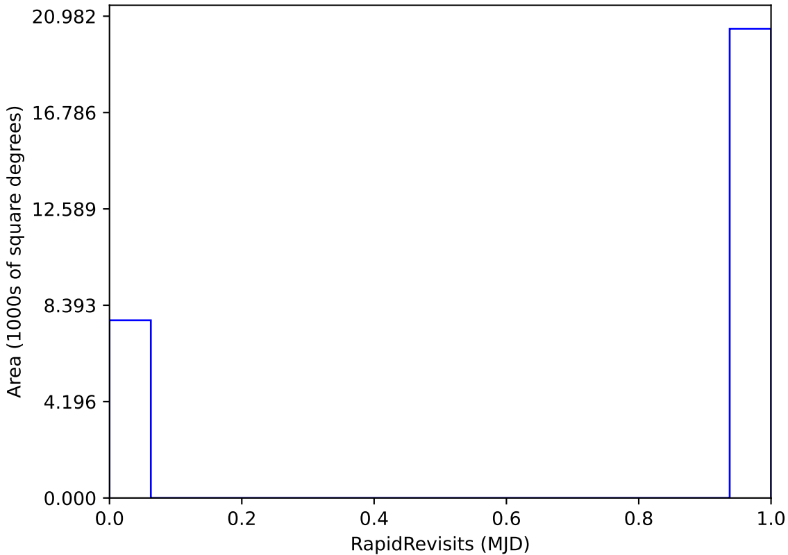
too_elab_r32_d3_griz_v3.4_10yrs All sky: RapidRevisits
