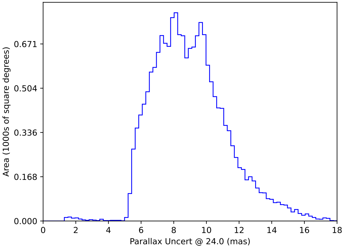
too_elab_r32_d3_griz_v3.4_10yrs WFD: Parallax Uncert @ 24.0
