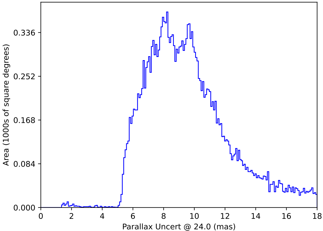
too_elab_r32_d3_griz_v3.4_10yrs All sky: Parallax Uncert @ 24.0
