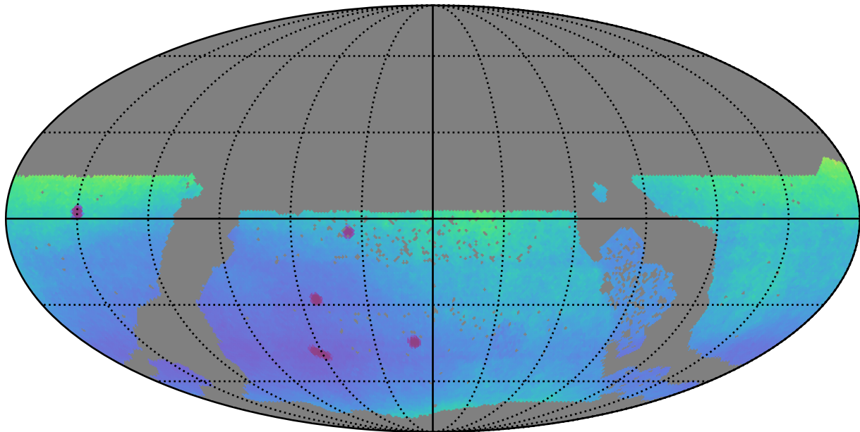
too_elab_r32_d3_griz_v3.4_10yrs WFD: Parallax Uncert @ 22.4
