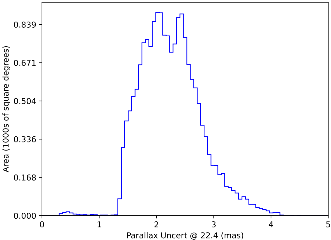
too_elab_r32_d3_griz_v3.4_10yrs WFD: Parallax Uncert @ 22.4
