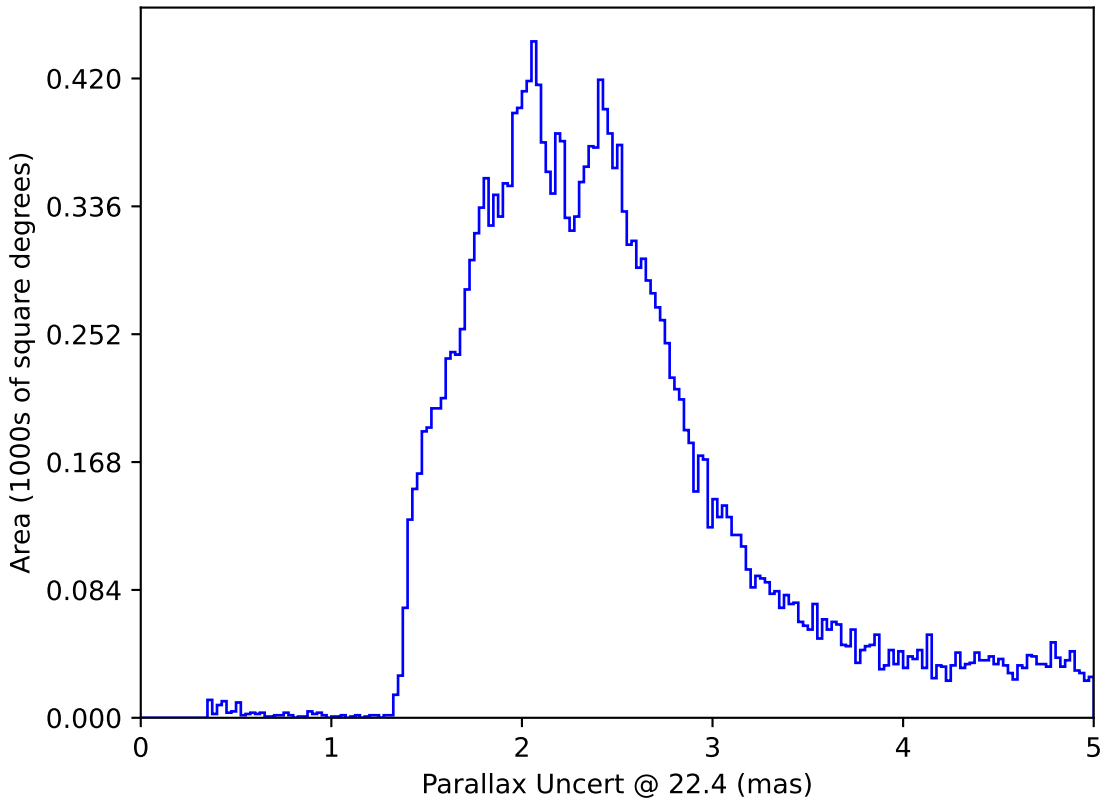
too_elab_r32_d3_griz_v3.4_10yrs All sky: Parallax Uncert @ 22.4
