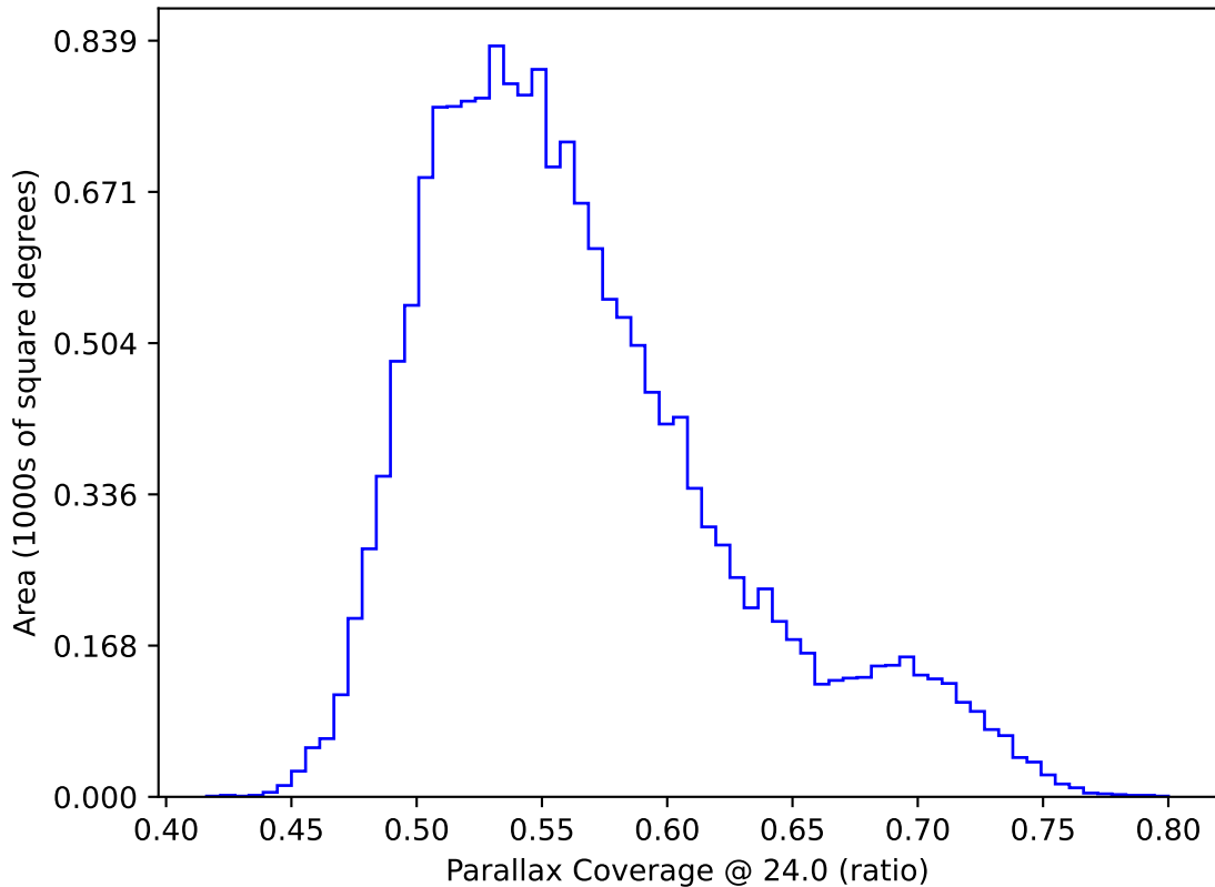
too_elab_r32_d3_griz_v3.4_10yrs WFD: Parallax Coverage @ 24.0
