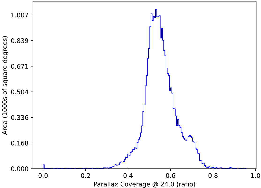
too_elab_r32_d3_griz_v3.4_10yrs All sky: Parallax Coverage @ 24.0
