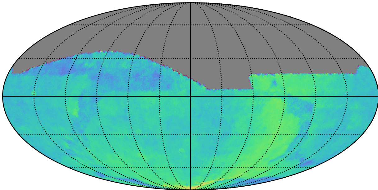
too_elab_r32_d3_griz_v3.4_10yrs All sky: Parallax Coverage @ 22.4
