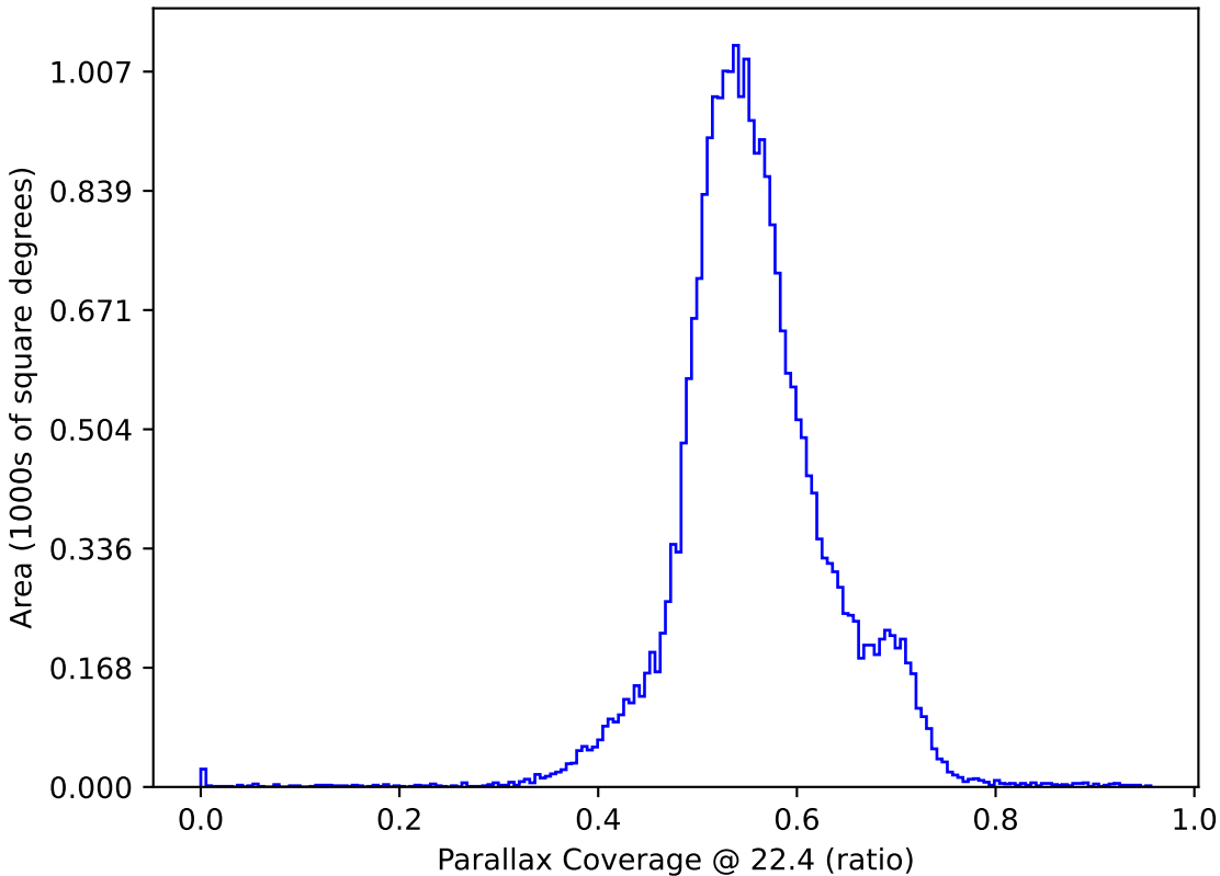
too_elab_r32_d3_griz_v3.4_10yrs All sky: Parallax Coverage @ 22.4
