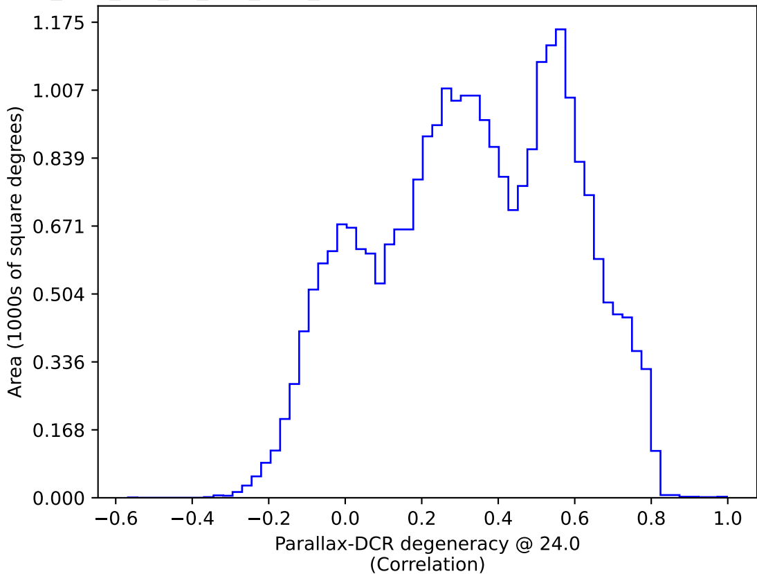
too_elab_r32_d3_griz_v3.4_10yrs All sky: Parallax-DCR degeneracy @ 24.0
