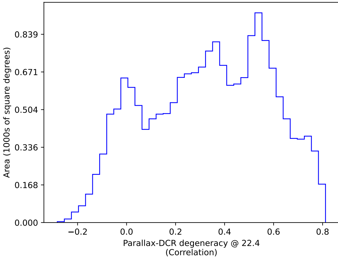
too_elab_r32_d3_griz_v3.4_10yrs WFD: Parallax-DCR degeneracy @ 22.4
