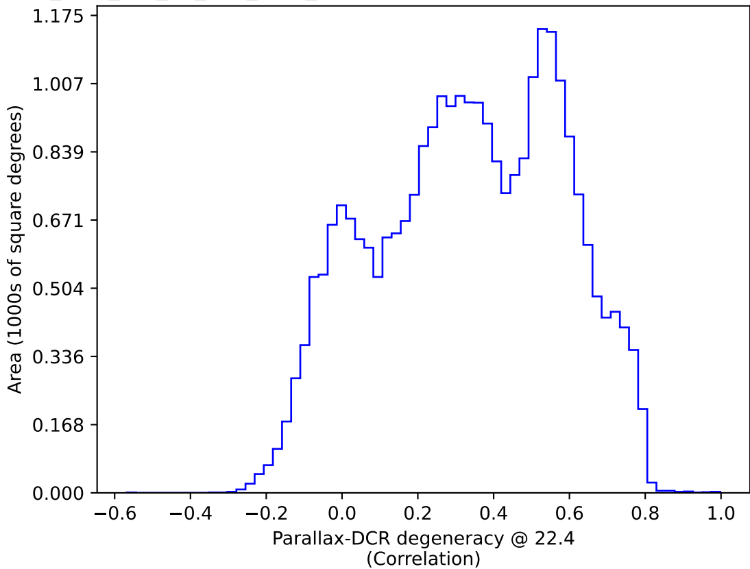
too_elab_r32_d3_griz_v3.4_10yrs All sky: Parallax-DCR degeneracy @ 22.4
