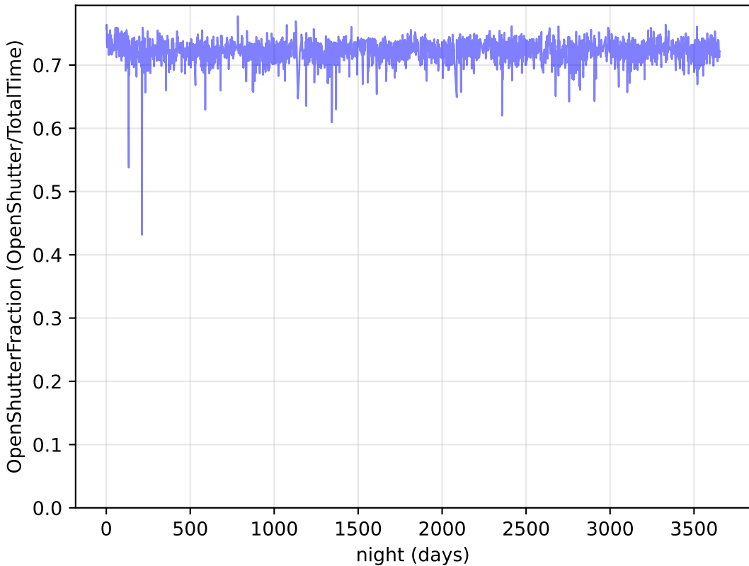
too_elab_r32_d3_griz_v3.4_10yrs Per night: OpenShutterFraction
