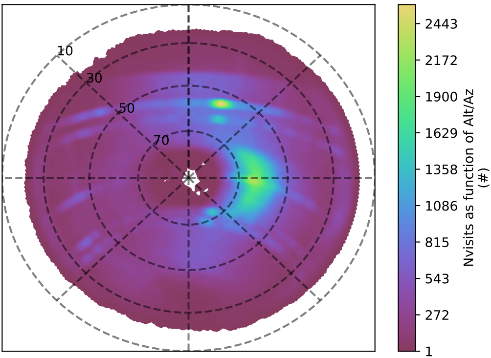
too_elab_r32_d3_griz_v3.4_10yrs z band: Nvisits as function of Alt/Az
