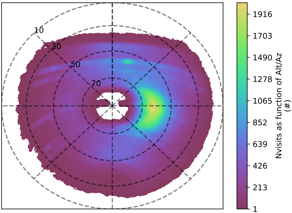
too_elab_r32_d3_griz_v3.4_10yrs y band: Nvisits as function of Alt/Az
