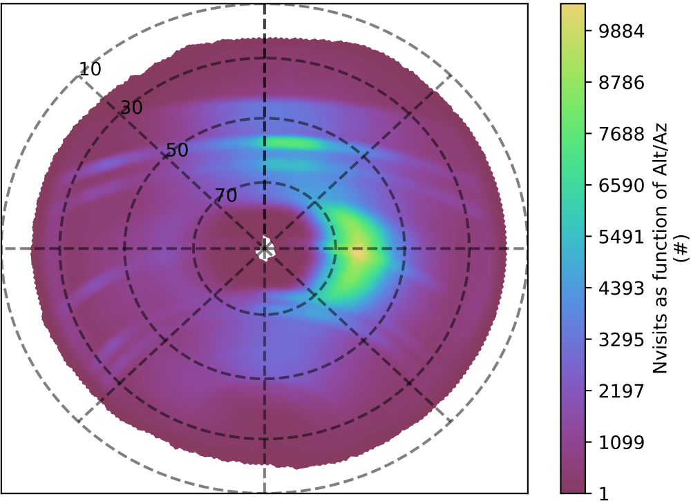
too_elab_r32_d3_griz_v3.4_10yrs all bands: Nvisits as function of Alt/Az
