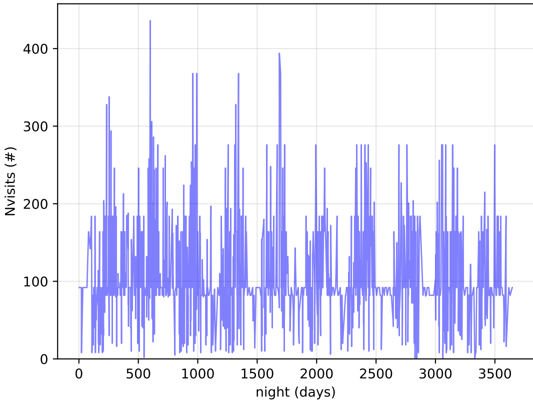
too_elab_r32_d3_griz_v3.4_10yrs DDF: Nvisits
