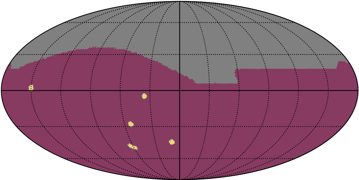
too_elab_r32_d3_griz_v3.4_10yrs All sky: NumberOfQuickRevisits
