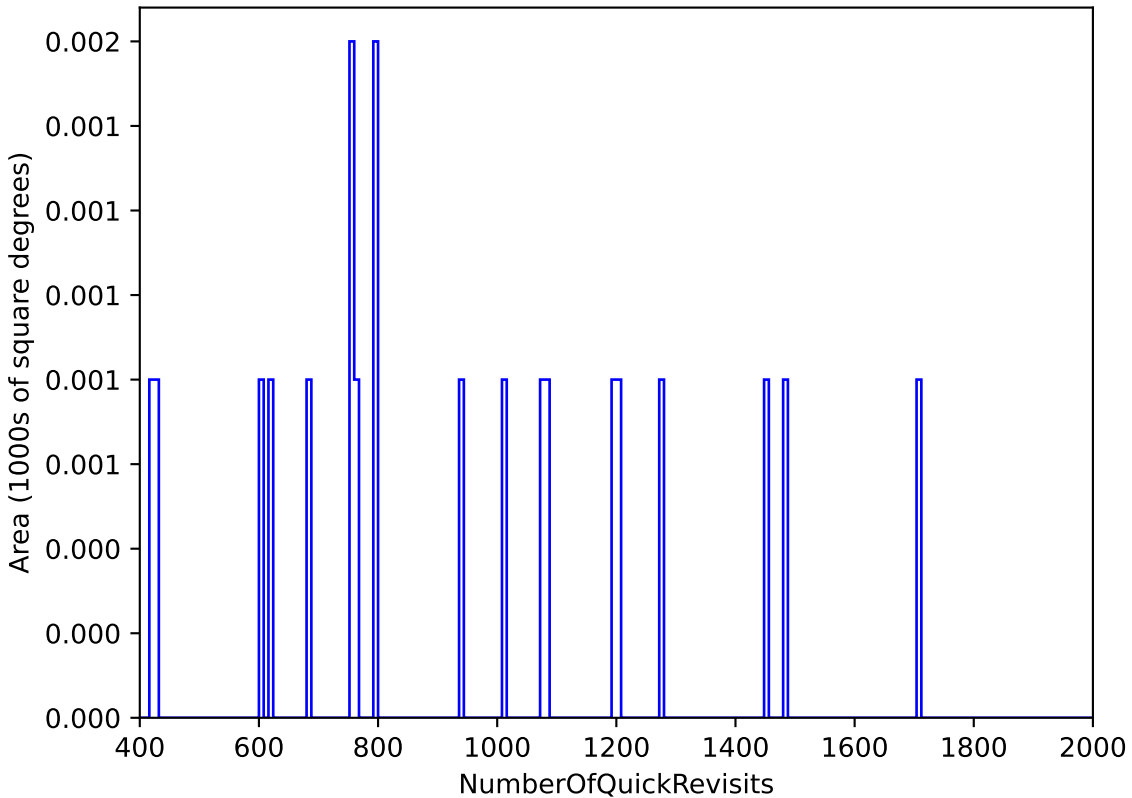
too_elab_r32_d3_griz_v3.4_10yrs All sky: NumberOfQuickRevisits
