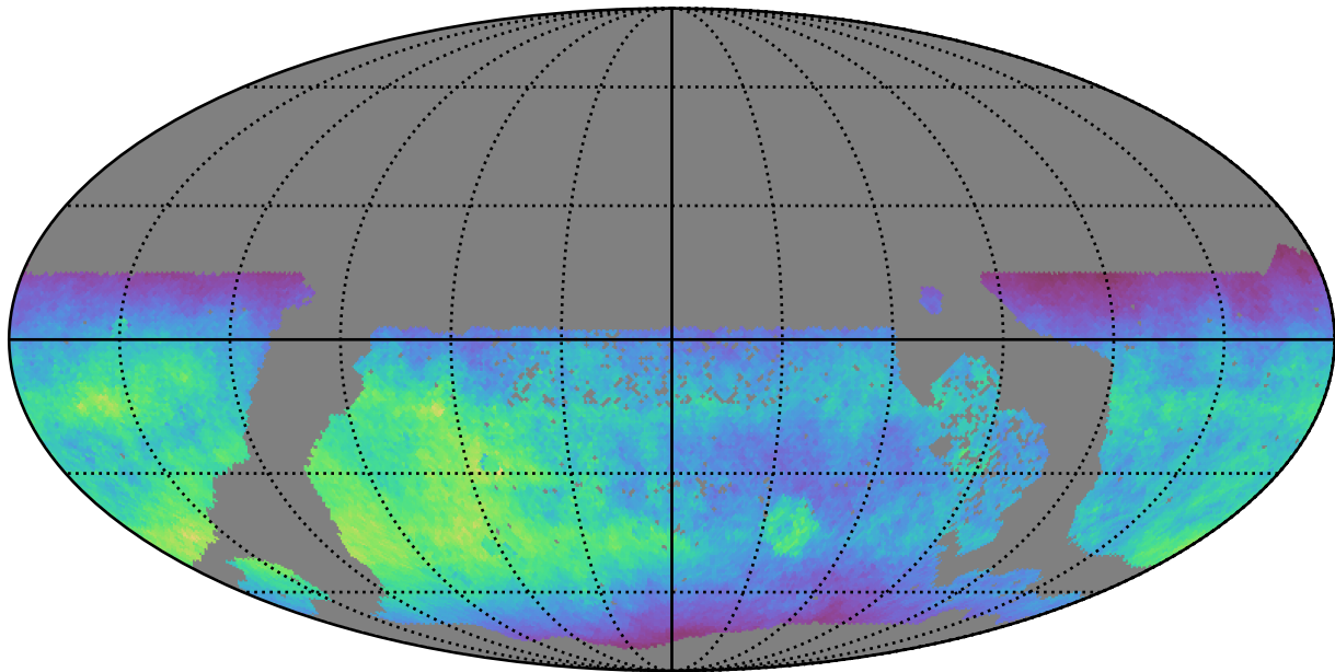
too_elab_r32_d3_griz_v3.4_10yrs WFD z band: Normalized Teff
