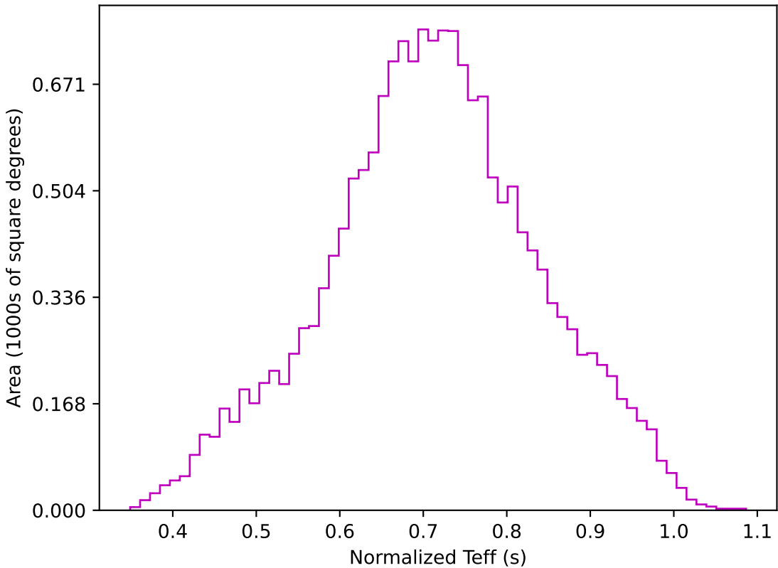
too_elab_r32_d3_griz_v3.4_10yrs WFD z band: Normalized Teff
