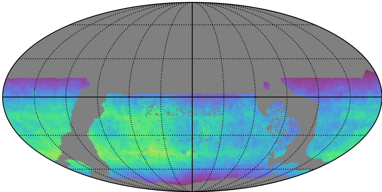
too_elab_r32_d3_griz_v3.4_10yrs WFD y band: Normalized Teff
