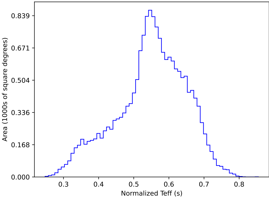
too_elab_r32_d3_griz_v3.4_10yrs WFD y band: Normalized Teff
