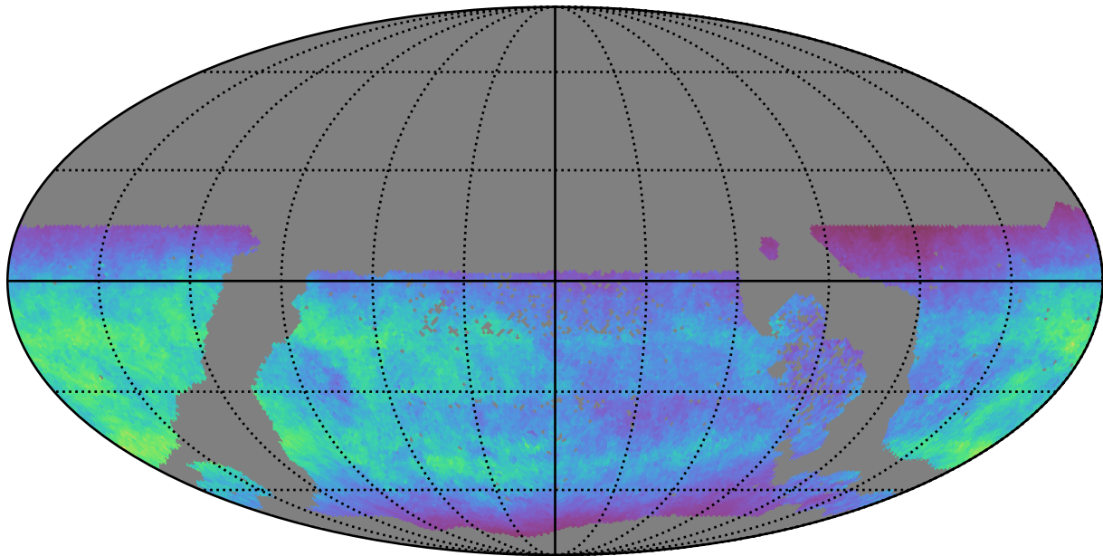
too_elab_r32_d3_griz_v3.4_10yrs WFD u band: Normalized Teff
