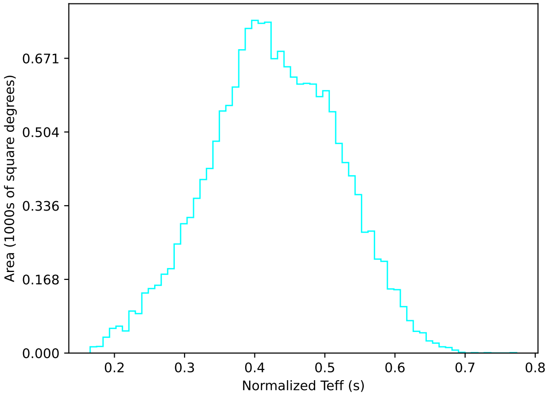
too_elab_r32_d3_griz_v3.4_10yrs WFD u band: Normalized Teff
