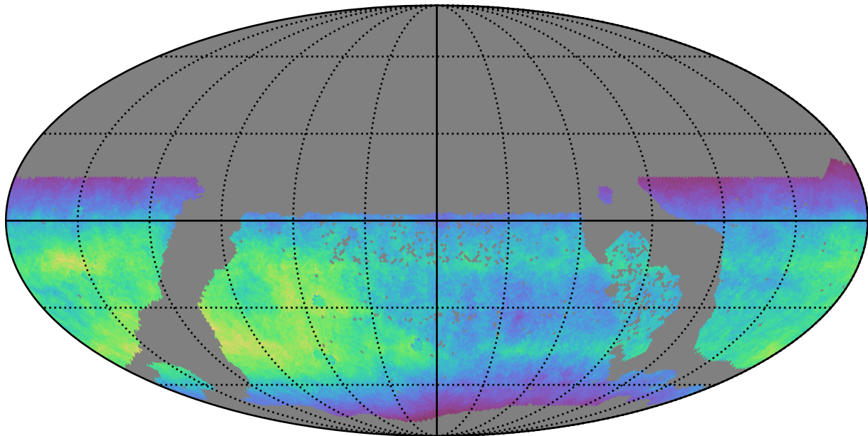
too_elab_r32_d3_griz_v3.4_10yrs WFD i band: Normalized Teff
