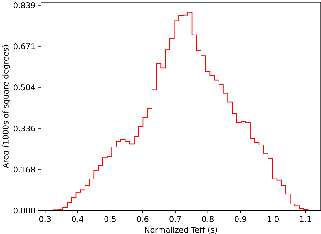
too_elab_r32_d3_griz_v3.4_10yrs WFD i band: Normalized Teff
