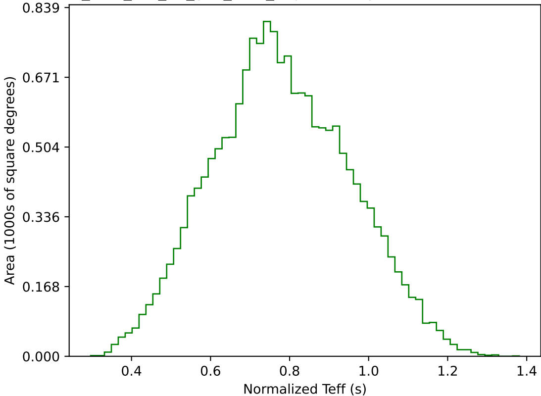
too_elab_r32_d3_griz_v3.4_10yrs WFD g band: Normalized Teff
