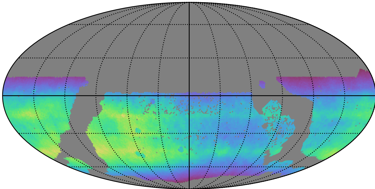
too_elab_r32_d3_griz_v3.4_10yrs WFD all bands: Normalized Teff
