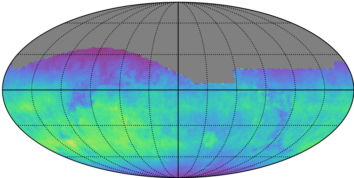
too_elab_r32_d3_griz_v3.4_10yrs All sky z band: Normalized Teff
