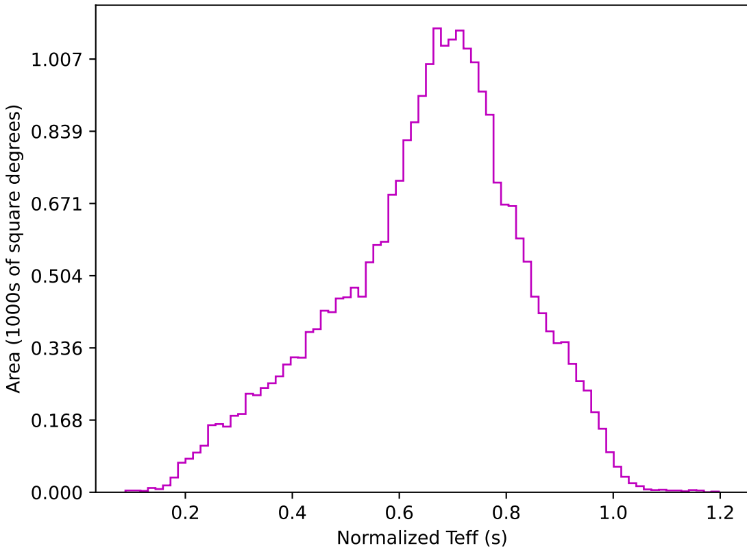
too_elab_r32_d3_griz_v3.4_10yrs All sky z band: Normalized Teff
