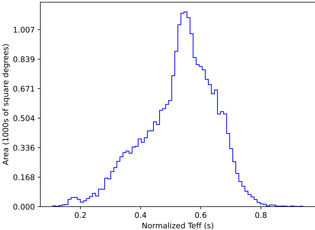
too_elab_r32_d3_griz_v3.4_10yrs All sky y band: Normalized Teff
